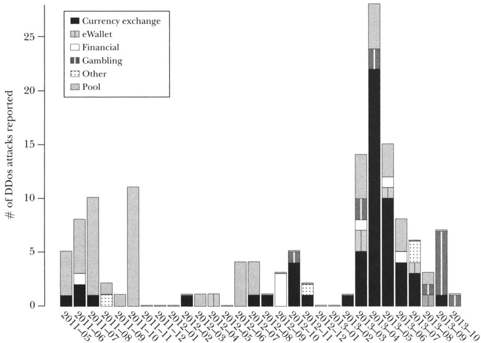
Figure 3 Reported (Distributed Denial of Service) DDoS Attacks on Bitcoin Services over Time
