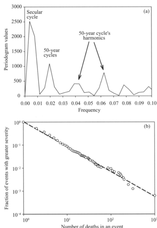
Figure 4. Statistical analyses
